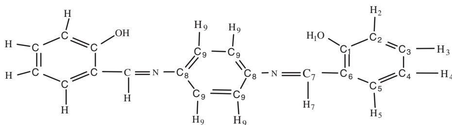
Figure 2. Structure of ligand.
